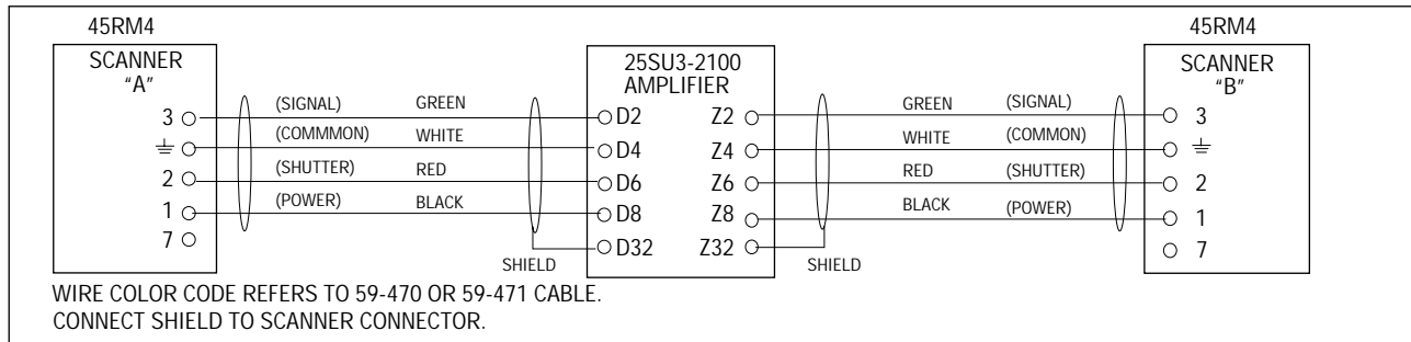
FIGURE 19 WIRING COMBINATIONS TO 60-2478 CONNECTOR, USED WITH CARD RACK FOR 25SU3-2000/2100 FLAME AMPLIFIERS
