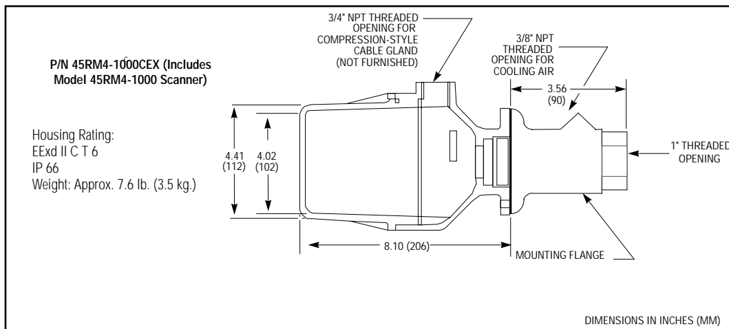
FIGURE 3 45RM4 SCANNER IN CENELEC HAZARDOUS AREA HOUSING
