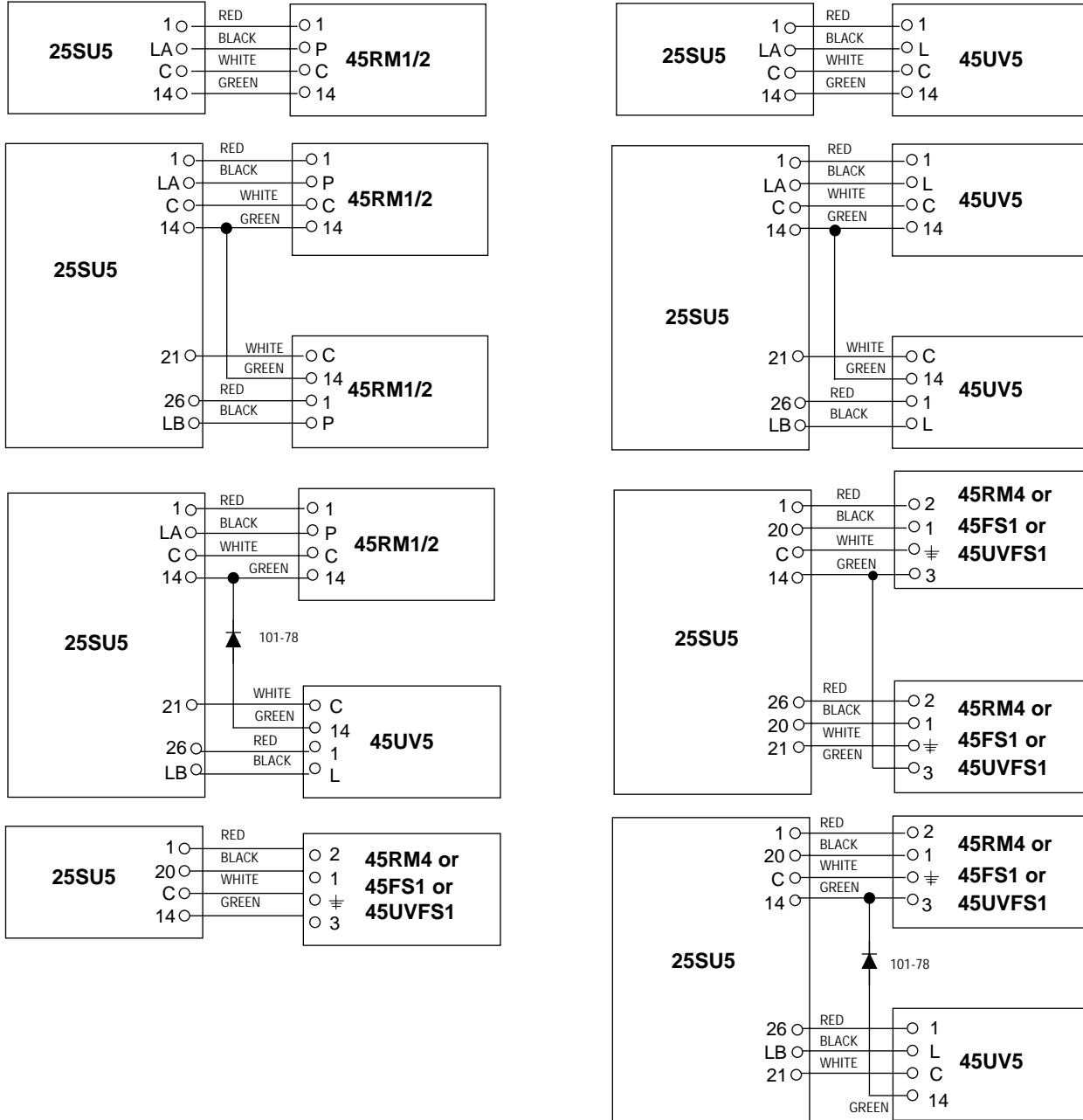
FIGURE 3. 25SU3-5166 or 25SU3-5168 Flame Safeguard Control Scanner(s) Wiring Combinations (see note 2)
