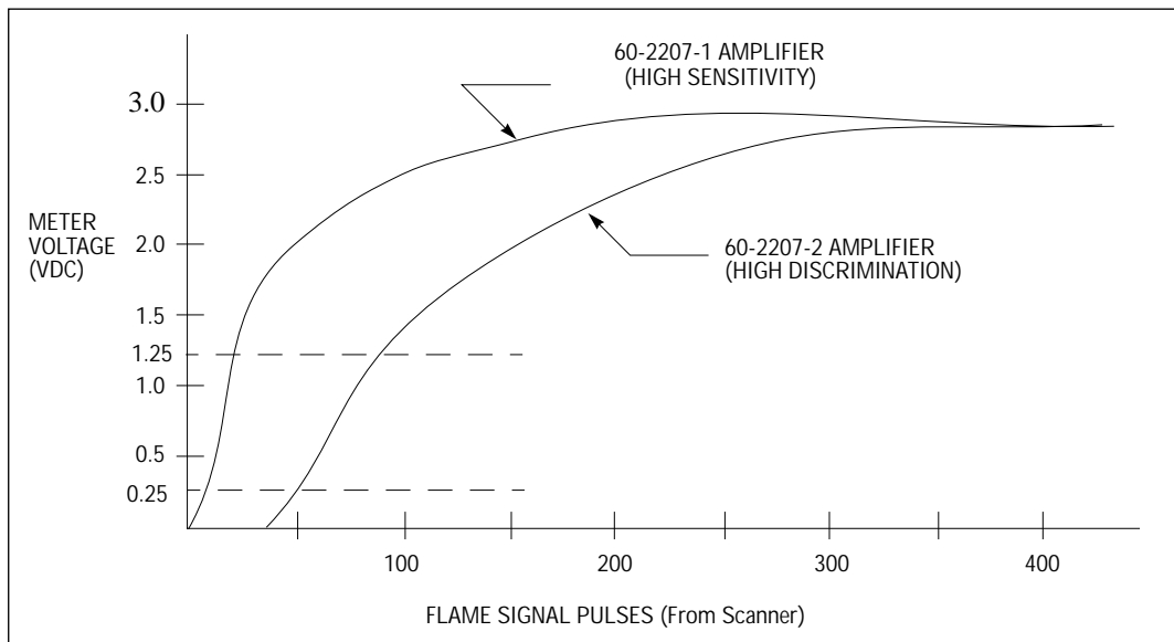
FIGURE 4. FLAME RESPONSE CURVES (shown with sensitivity set @ maximum)
