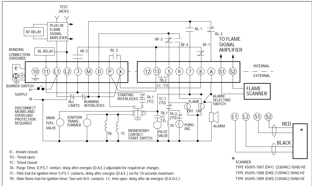
FIGURE 3. TYPICAL SCHEMATIC DIAGRAM FOR SEMI-AUTOMATIC PILOT IGNITED GAS OR OIL BURNER WITH PREPURGE, PILOT TFI, MAIN FLAME TFI AND INTERRUPTED PILOT
