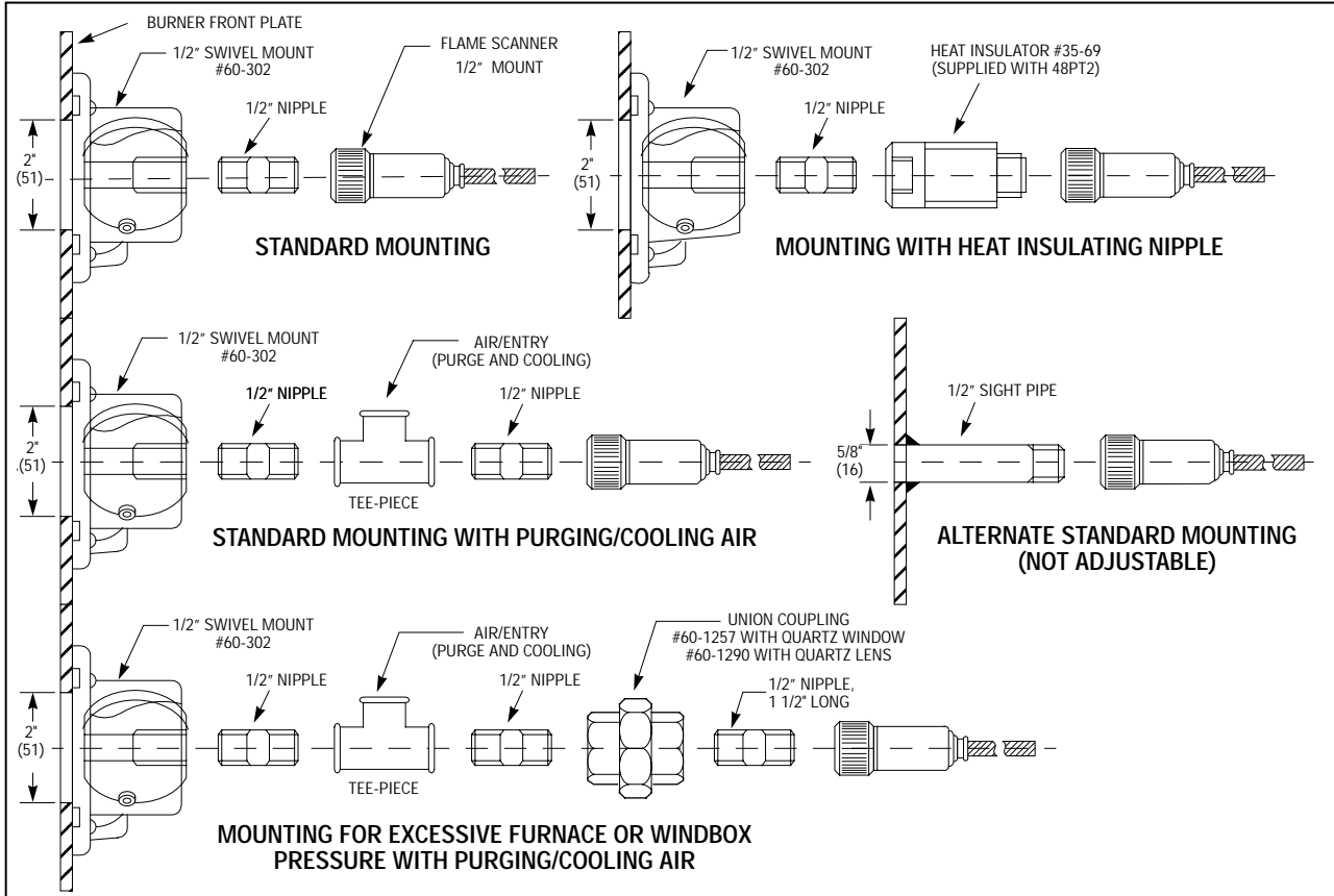
FIGURE 4. Mounting UV1A/48PT2 Scanners
